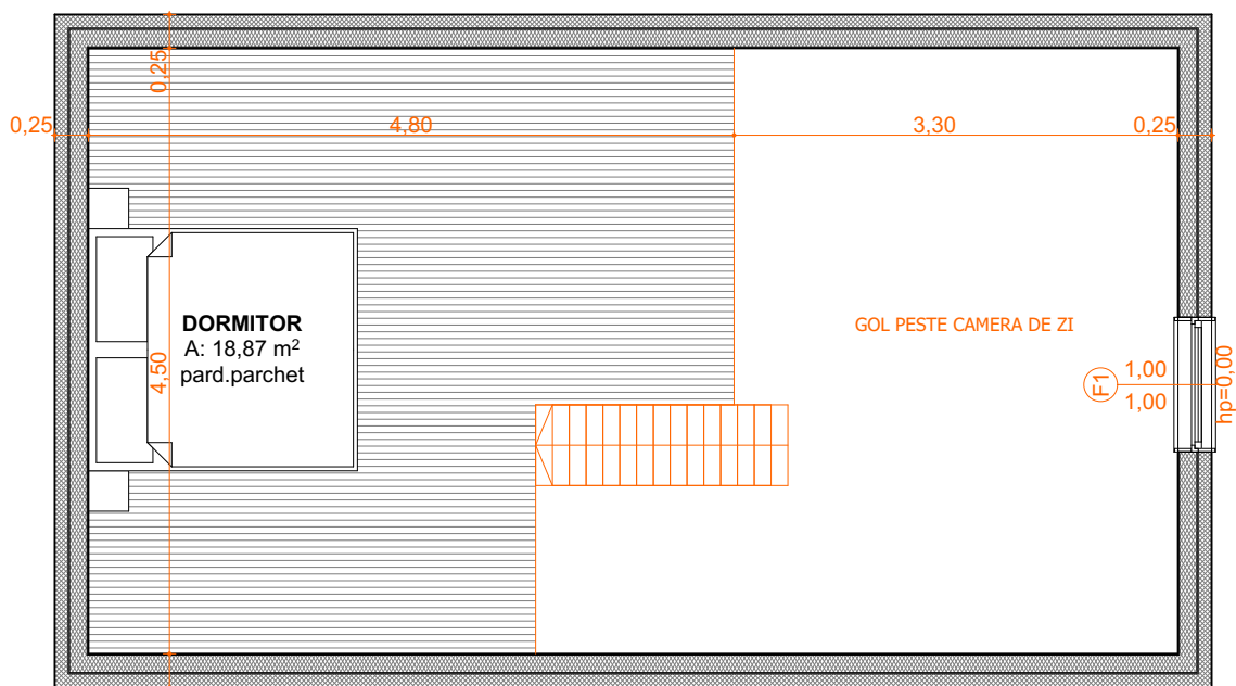
PLAN MANSARDA
